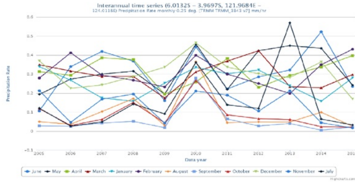
Fig. 2 Average Monthly Rainfall of TRMM, Time Series
