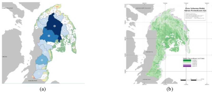
Fig. 4 (a) Area Catchment Numbers and (b) Map of Surface Flow Discharge Distribution
