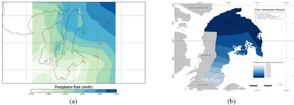
Fig. 3 (a) TRMM Data in the Form of Distribution Map and (b) Grid Rain Intensity Grid
